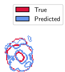
segmentations
